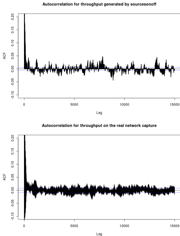
Figure 9. Generated (top) vs. real (bottom) throughput autocorrelations
