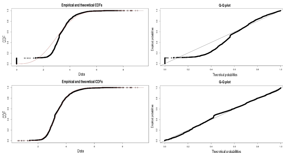
Figure 4. Example of traffic decomposition (ECDF [left] and QQPlot [right] functions for real data [top] and Weibull distribution [bottom])
