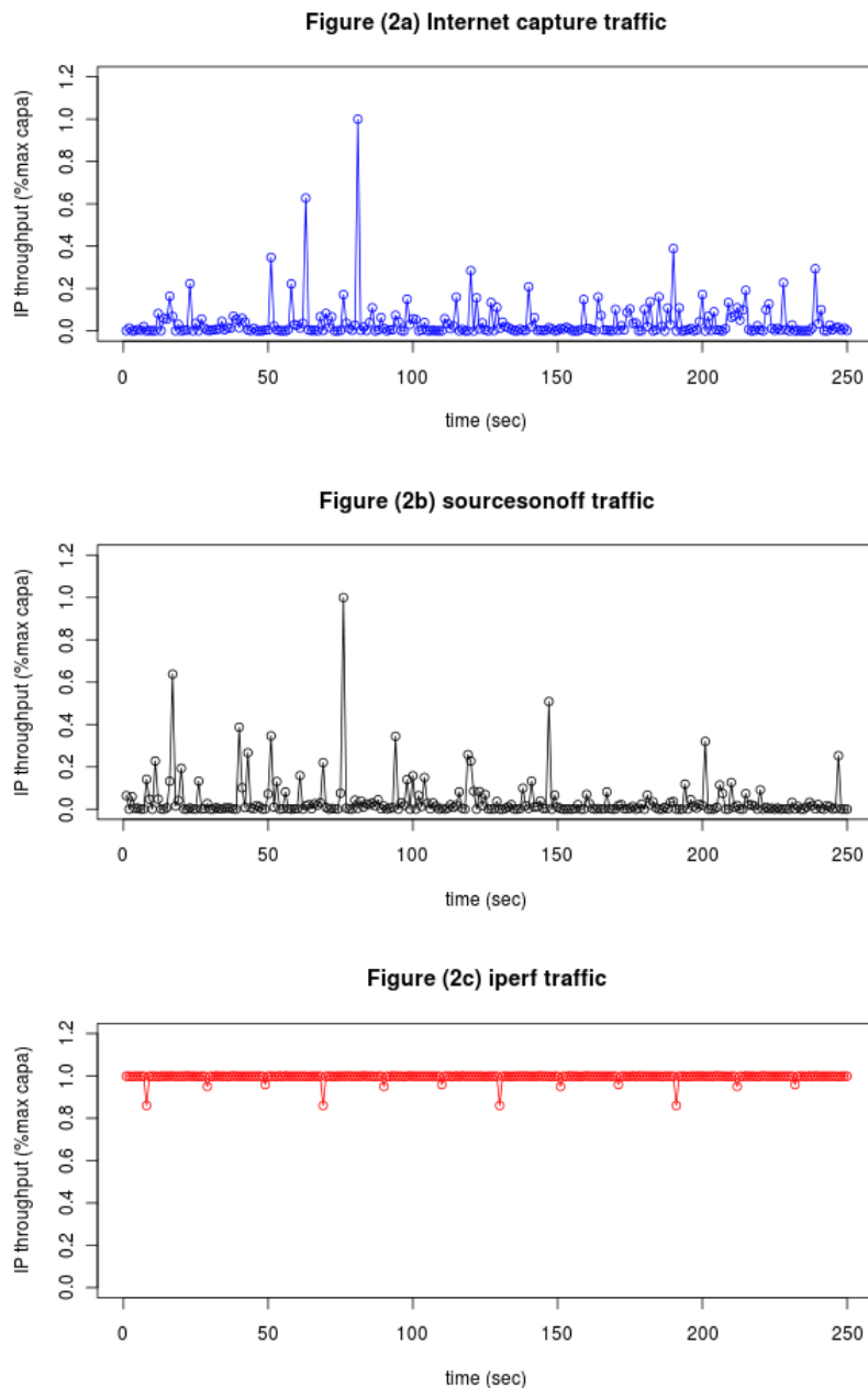
Figure 2. Throughputs generated by iperf and our tool
