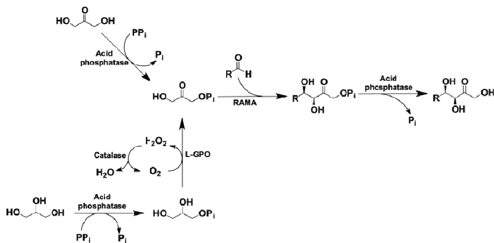
Figure 1. Scheme of the one-pot cascade reactions starting from DHA or glycerol at pH 6
