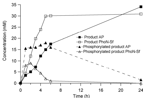
Figure 5. Time course of the formation of product and phosphorylated product in the two-enzyme cascade reaction using immobilized AP or immobilized PhoN-Sf. Reaction mixtures contain 500 mM DHA, 100 mM PP_i , 100 mM propanal, RAMA 6 U/mL, 20 U/mL immobilized AP at pH 8 or 1 U/mL immobilized PhoN-Sf at pH 6, at 30 °C
