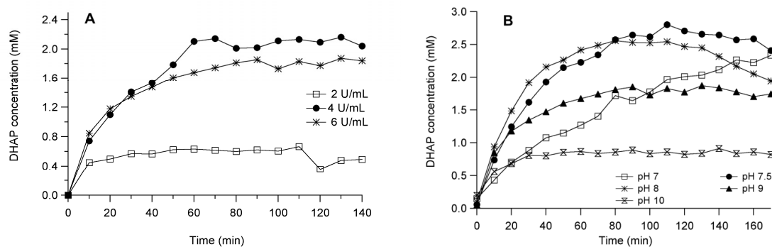
Figure 3. A) Time course of the phosphorylation of DHA by three different concentrations of AP (2, 4, and 6 U/mL). Reaction mixtures contains 100 mM DHA, 50 mM PP_i , at pH 9, at 30 °C. B) pH dependency of the phosphorylation of DHA. Reaction mixtures contains 100 mM DHA, 50 mM PP_i , 6 U/mL AP, at 30 °C, and pH values from 7 to 10
