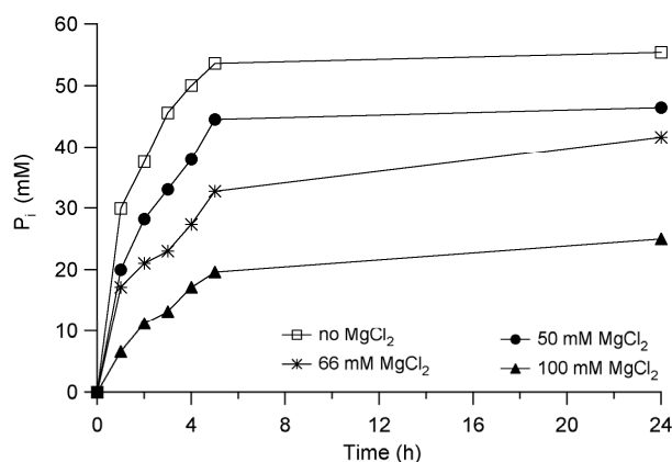
Figure 2. Rate of hydrolysis of PP_i in presence of various concentrations of MgCl_2 . Reaction mixtures contain 100 mM PP_i , 0, 50, 66, or 100 mM MgCl_2 , at pH 8, 30 °C. The PP_i/Mg^{2+} ratios are 2:1 for 50 mM MgCl_2 , 3:2 for 66 mM MgCl_2 , and 1:1 for 100 mM MgCl_2
