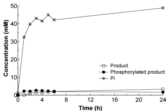
Figure 4. Time course of the two-enzyme cascade reaction using soluble AP. The reaction mixture contains 100 mM PP_i , 500 mM DHA, 100 mM propanal, 6 U/mL AP, 6 U/mL RAMA, pH 8 at 30 °C
