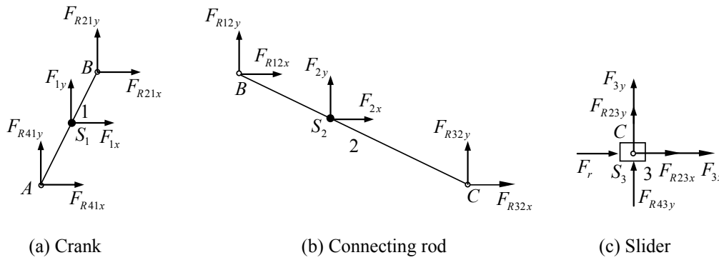
Figure 4. Force analysis of each component
