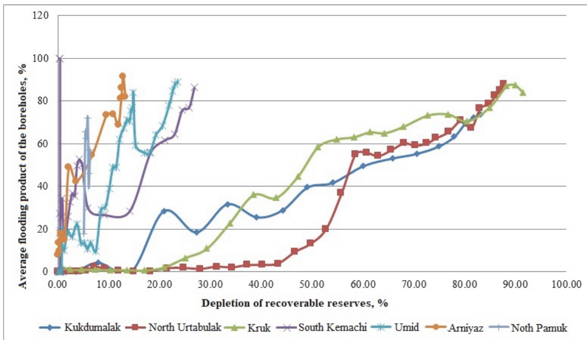
Figure 2. Dynamics of average water-cut of well production due to depletion of recoverable reserves
