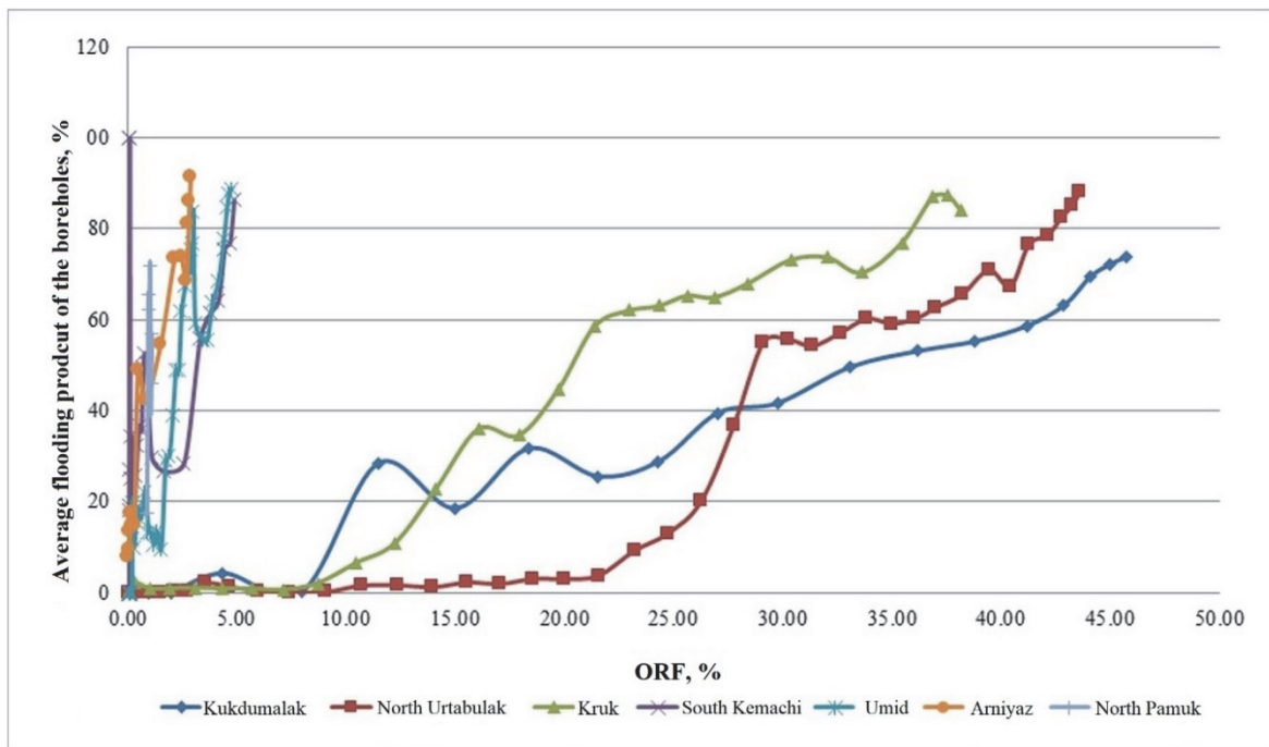
Figure 3. Dynamics of average water cut of wells from the current oil recovery ratio the reasons for their differences with the use of multivariate correlation analysis
